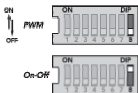
Figura 2.01 Interruptor # 8
